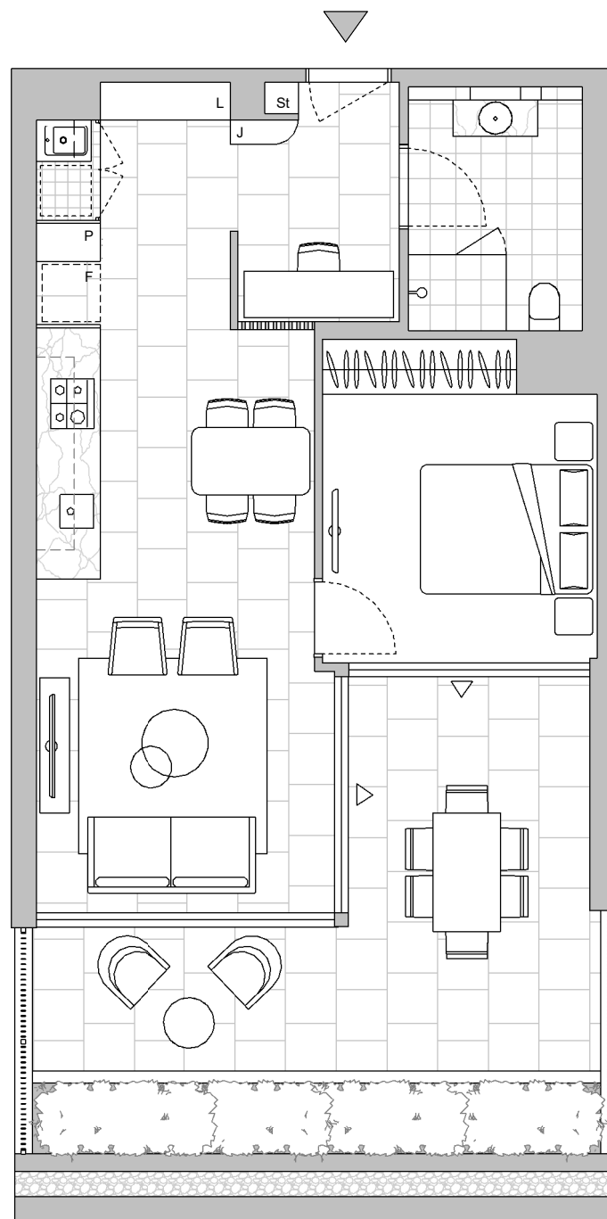
LEVEL B1
